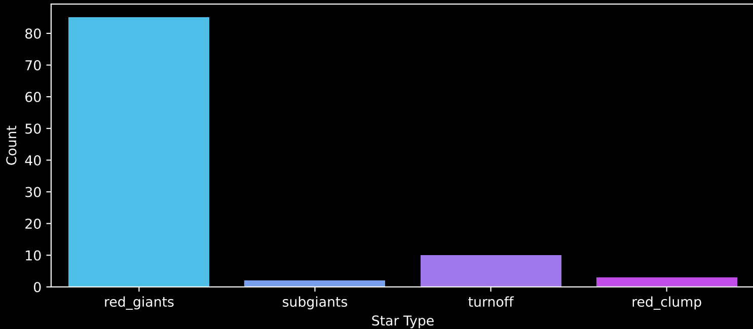
APOGEE DR17 Field: [LMC20] Count plot of Star Type
