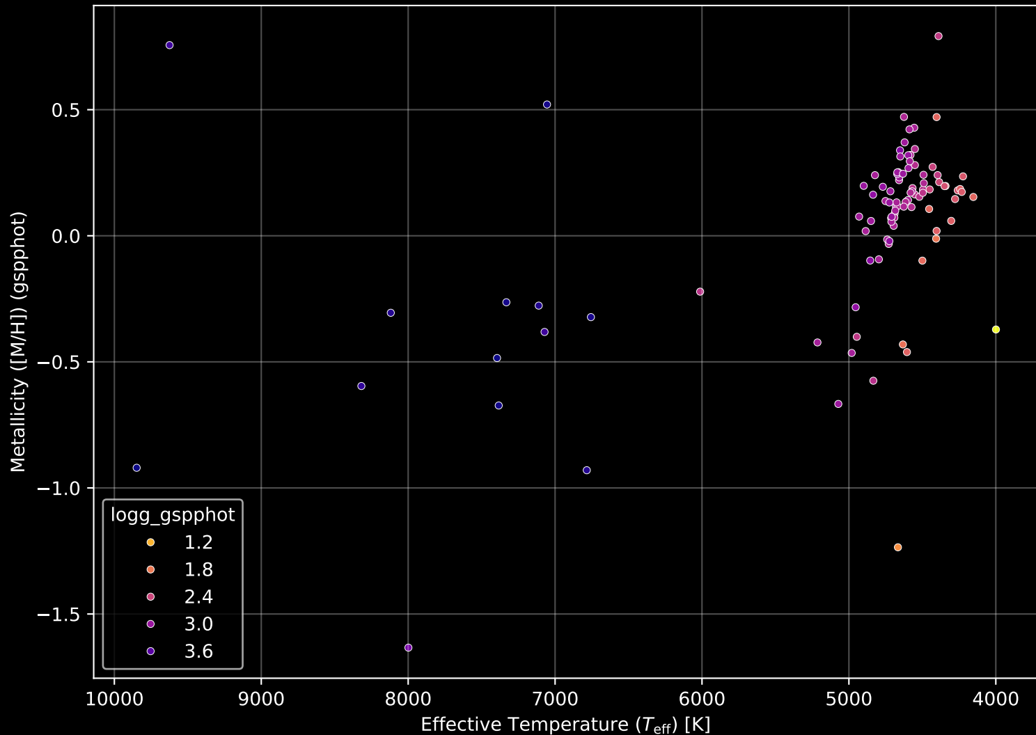
APOGEE DR17 Field: [LMC20] Stellar Population Parameters (n= 100)
