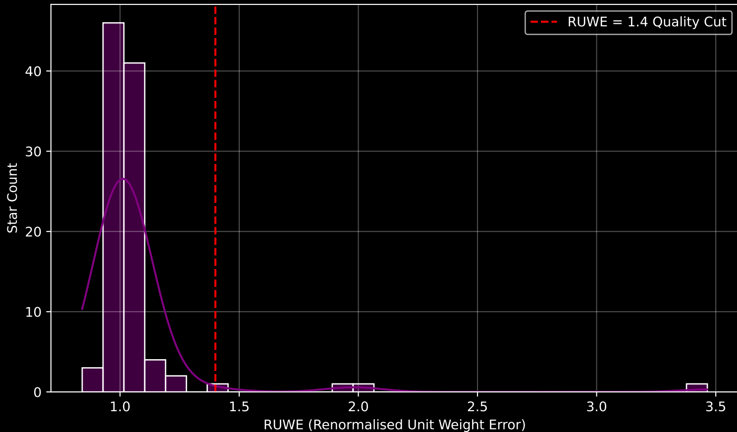
GAPOGEE DR17 Field [LMC20] RUWE Distribution (n= 100)
