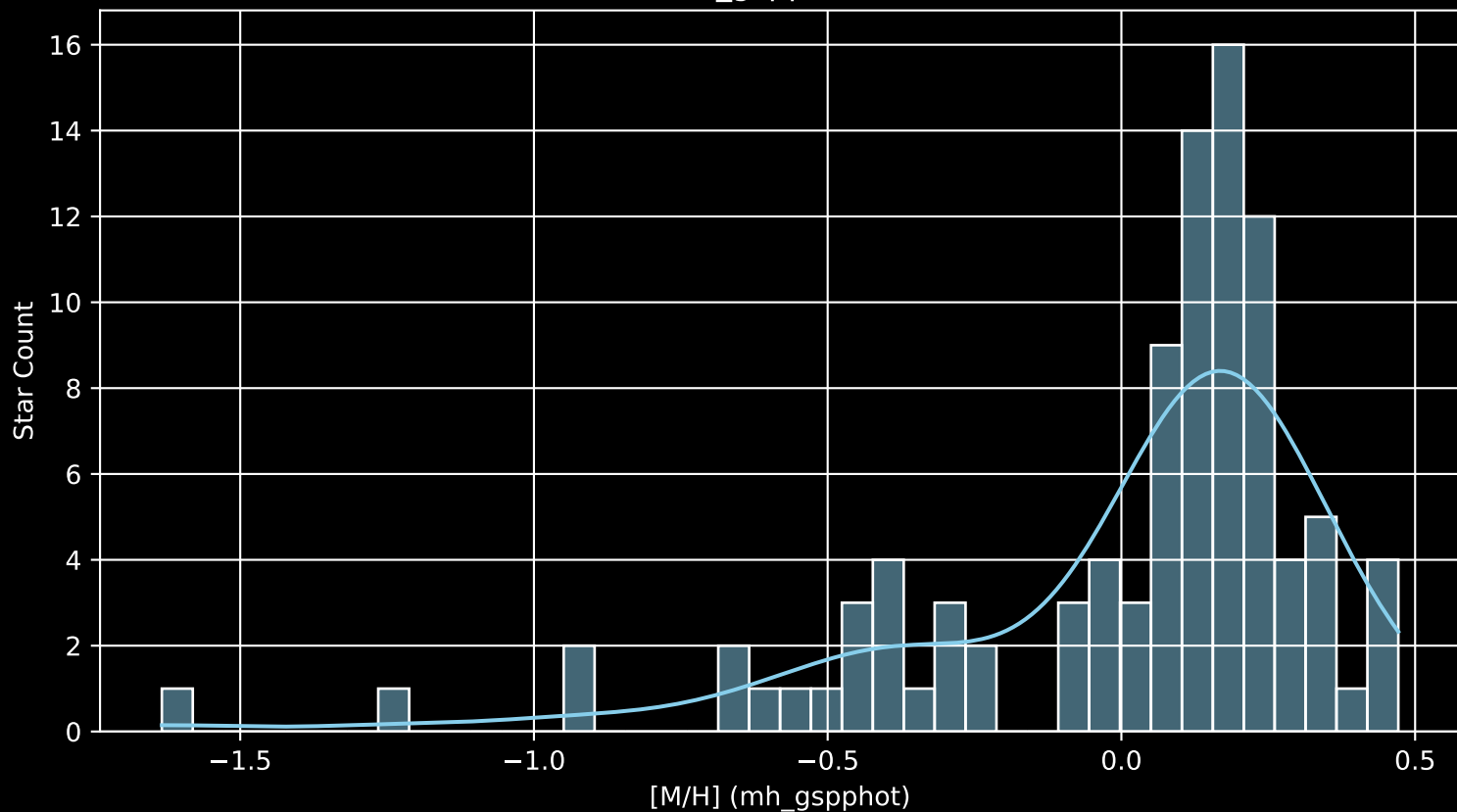
APOGEE DR17 Field: [LMC20 [M/H] (mh_gspphot) (n= 97)
