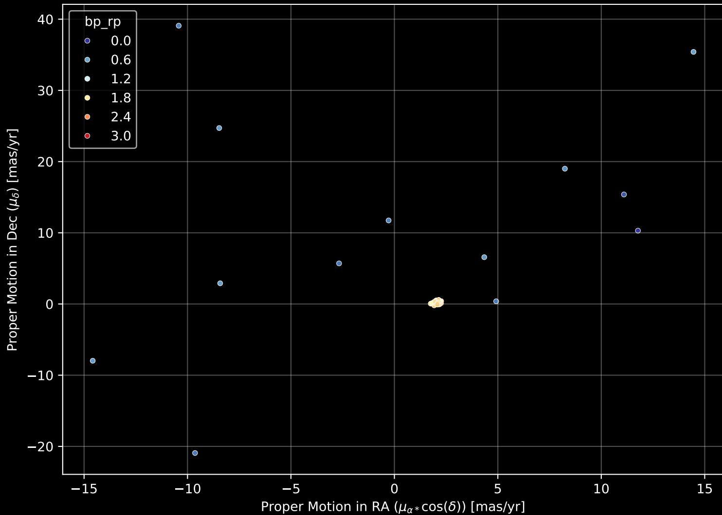
APOGEE DR17 Field: [LMC20] Proper Motion Diagram (n= 100)
