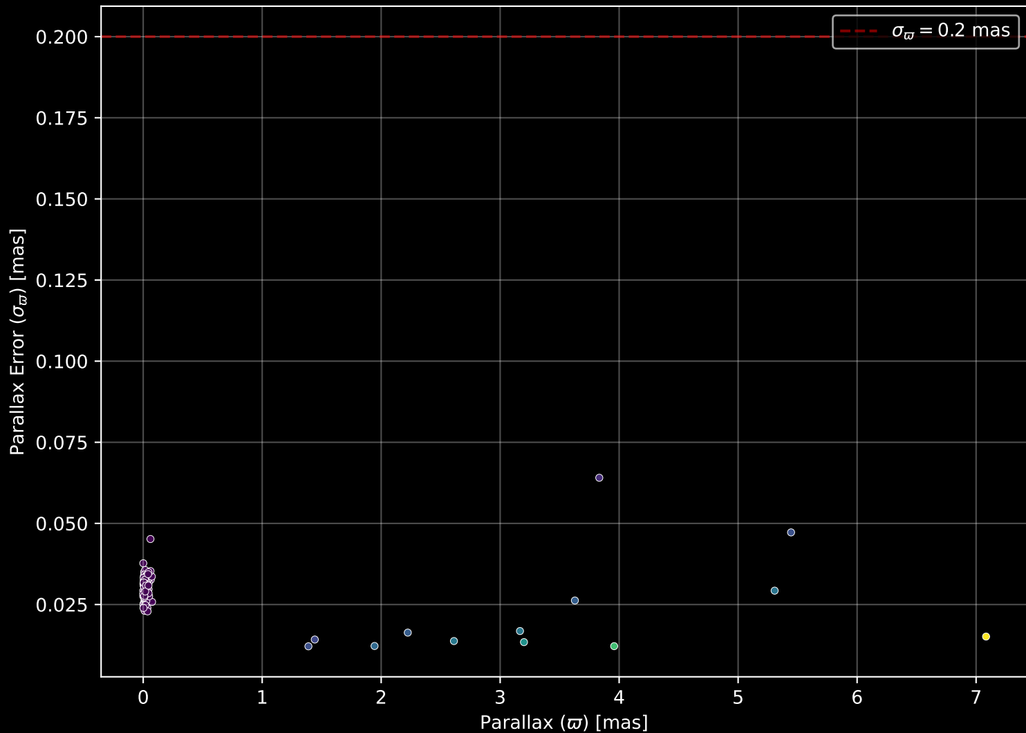
APOGEE DR17 Field: [LMC20] Parallax Quality (n= 100)
