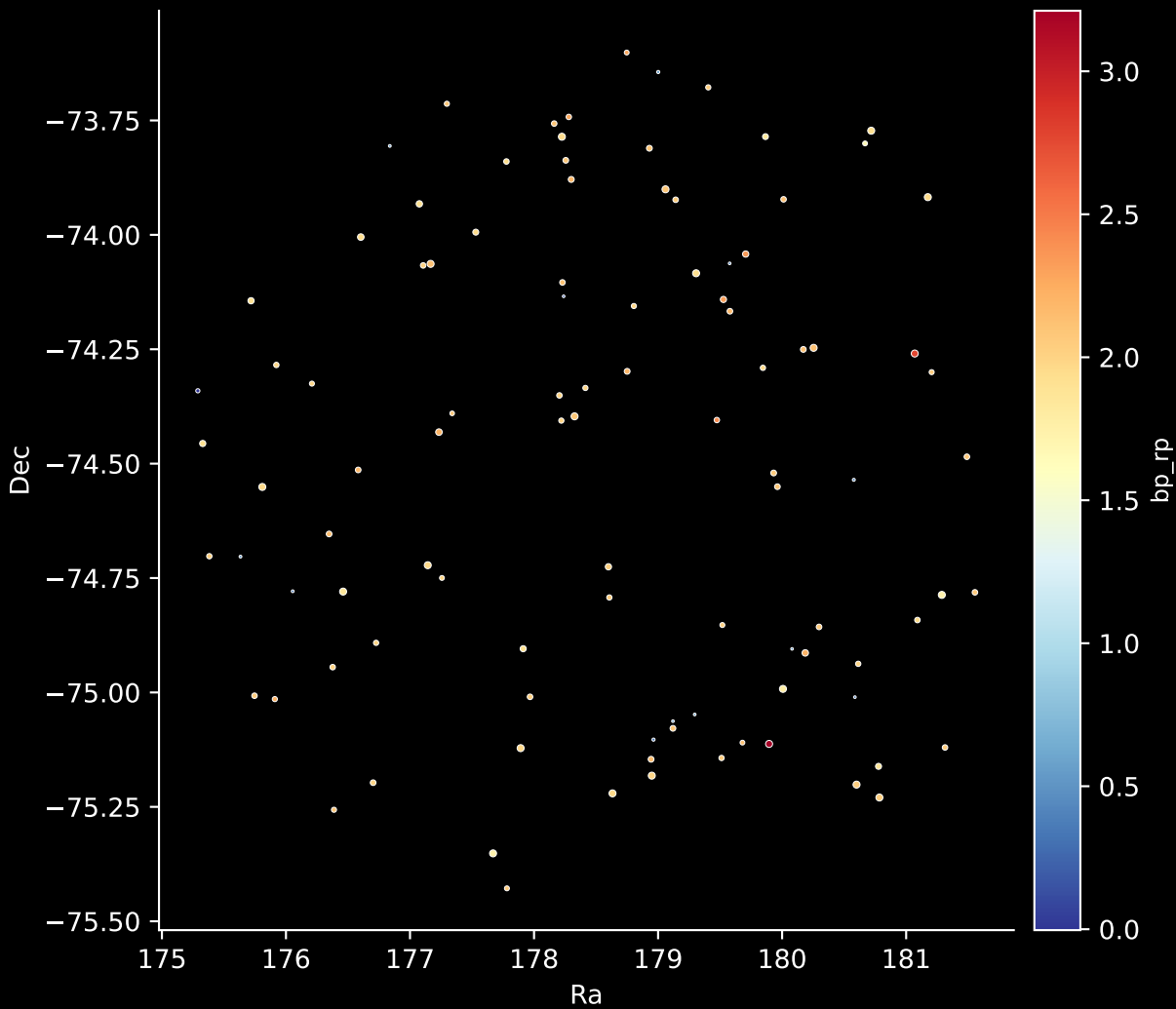
APOGEE DR17 Field: [LMC20] Stars: 100
